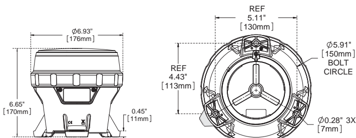
Total height including wireless antenna is 10.9" (276 mm)
